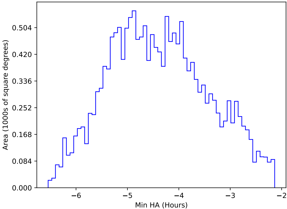
too_elab_heavy_r64_d2_griz_v3.4_10yrs WFD i band: Min HA
