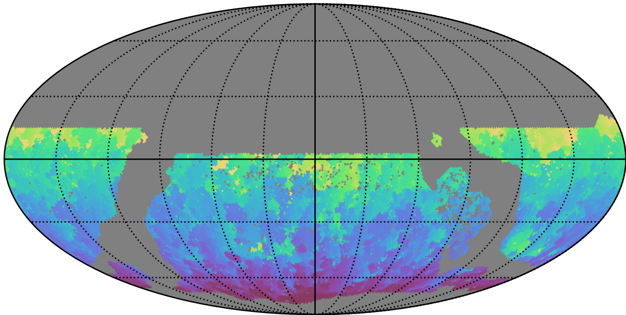
too_elab_heavy_r64_d2_griz_v3.4_10yrs WFD g band: Min HA
