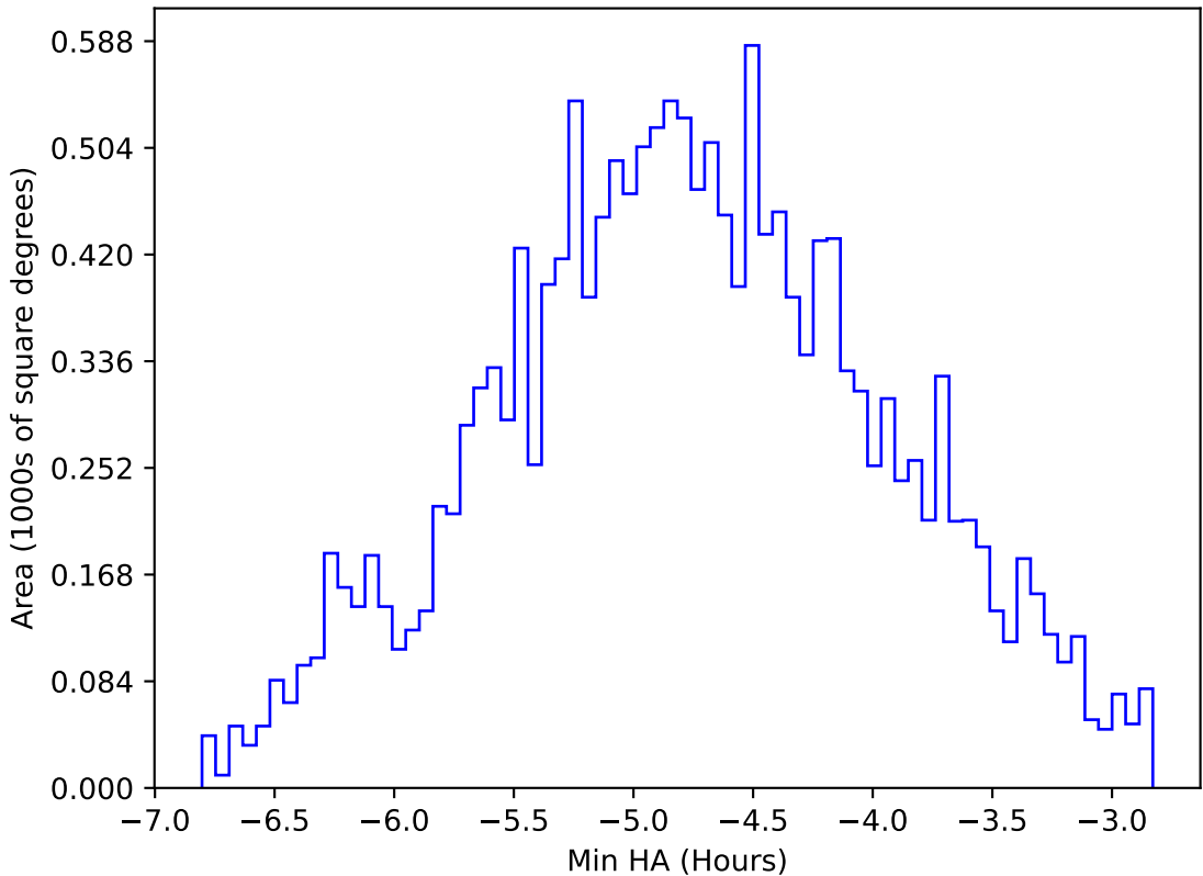
too_elab_heavy_r64_d2_griz_v3.4_10yrs WFD all bands: Min HA
