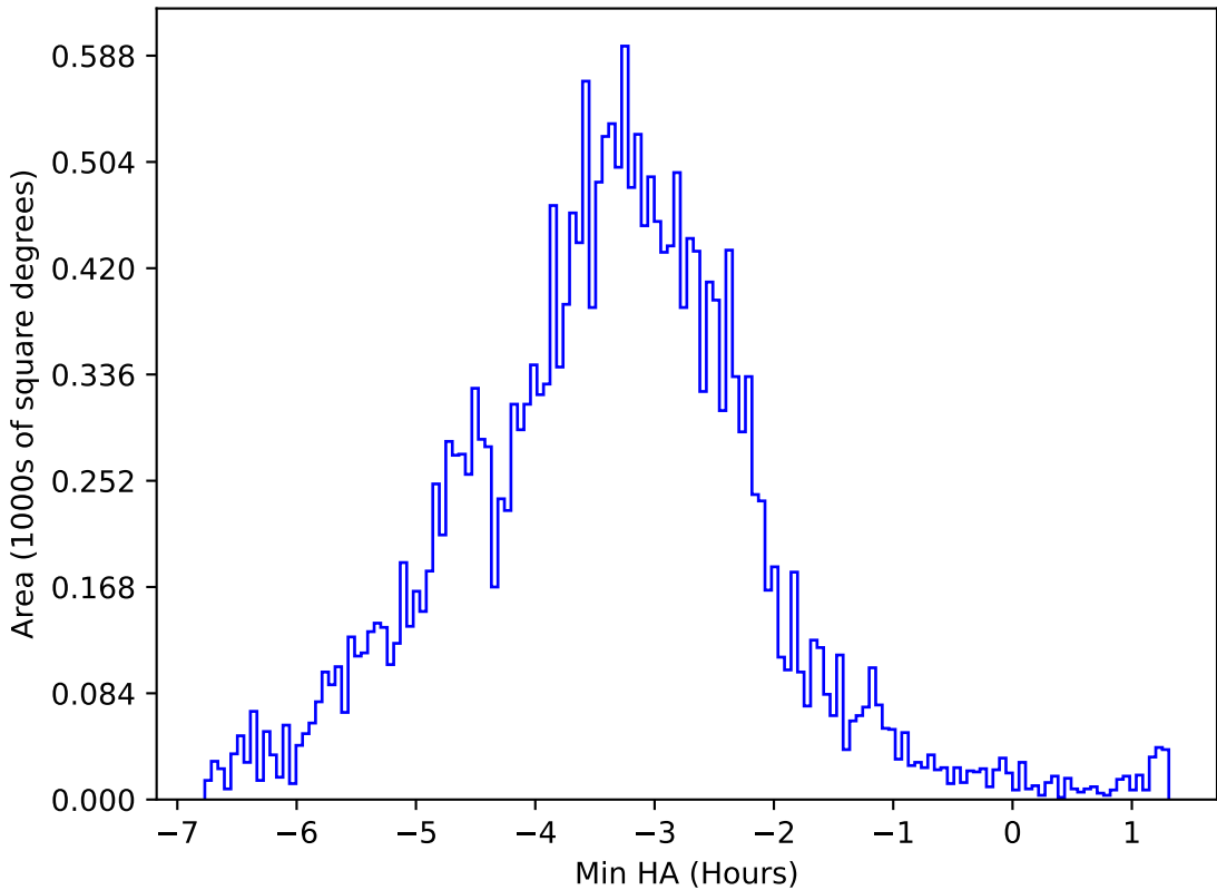
too_elab_heavy_r64_d2_griz_v3.4_10yrs All sky y band: Min HA
