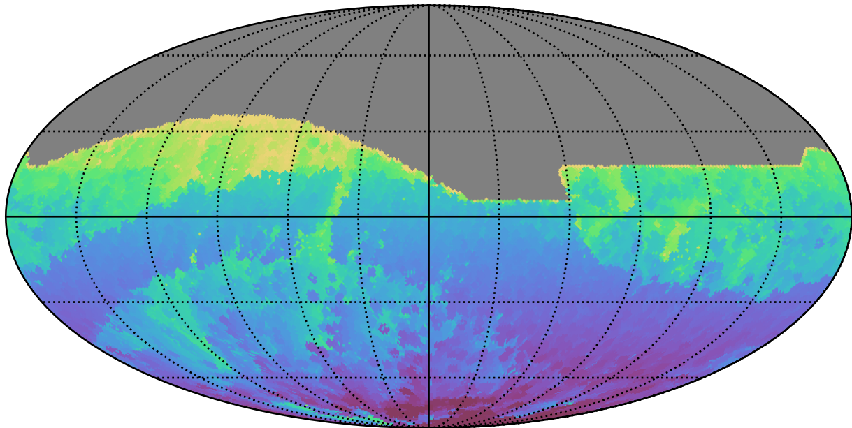
too_elab_heavy_r64_d2_griz_v3.4_10yrs All sky r band: Min HA
