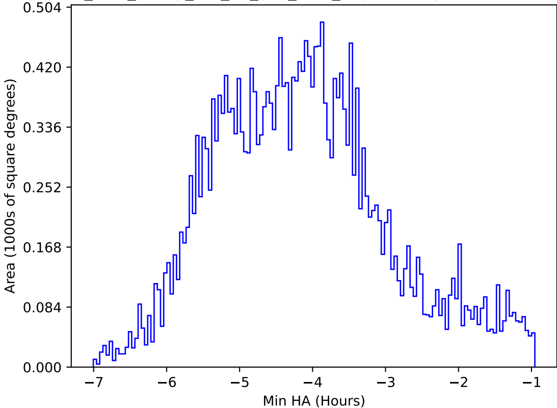
too_elab_heavy_r64_d2_griz_v3.4_10yrs All sky r band: Min HA
