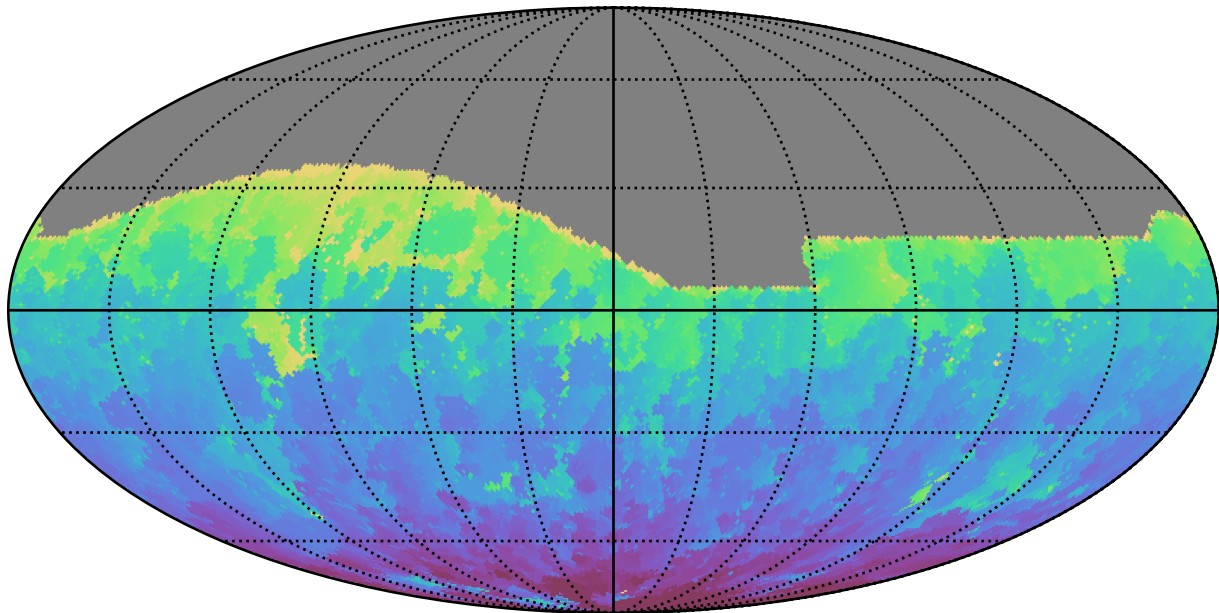
too_elab_heavy_r64_d2_griz_v3.4_10yrs All sky g band: Min HA
