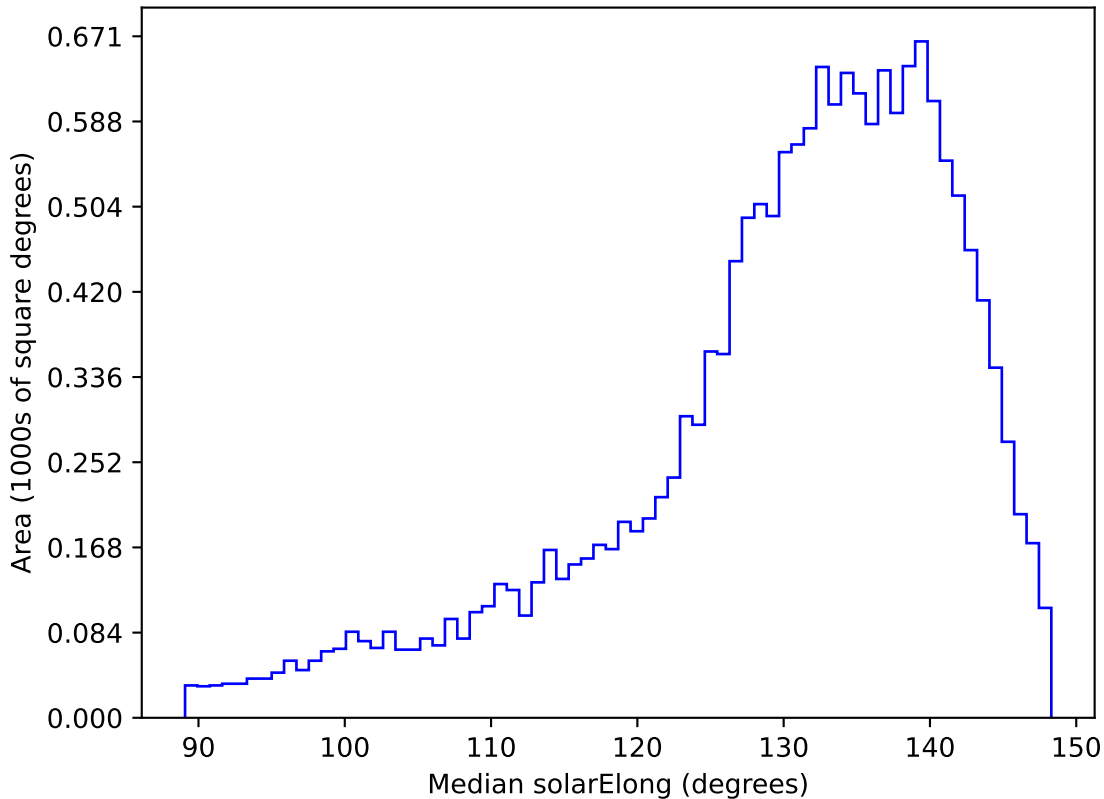
too_elab_heavy_r64_d2_griz_v3.4_10yrs WFD y band: Median solarElong
