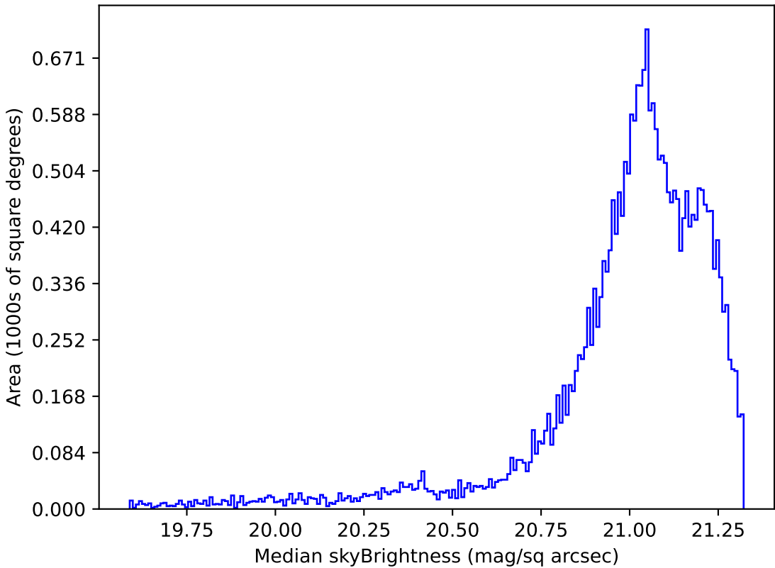
too_elab_heavy_r64_d2_griz_v3.4_10yrs Yr 1 r band: Median skyBrightness
