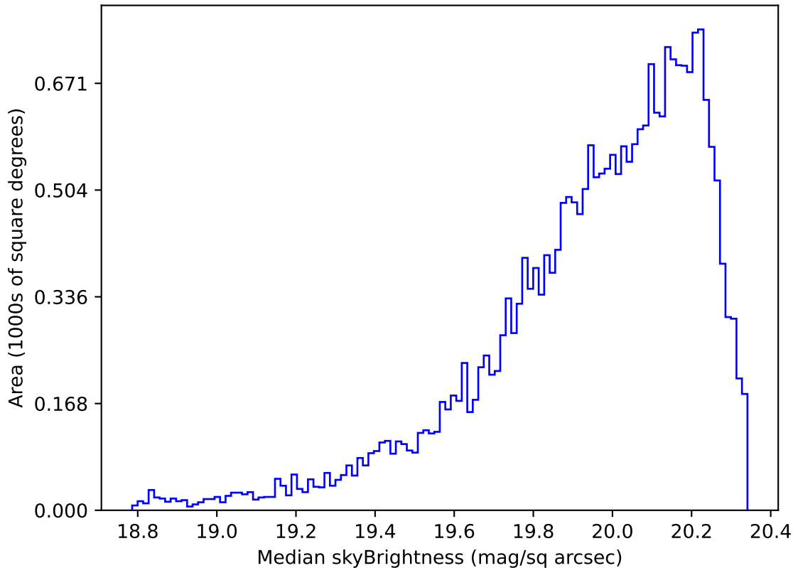
too_elab_heavy_r64_d2_griz_v3.4_10yrs Yr 1 i band: Median skyBrightness
