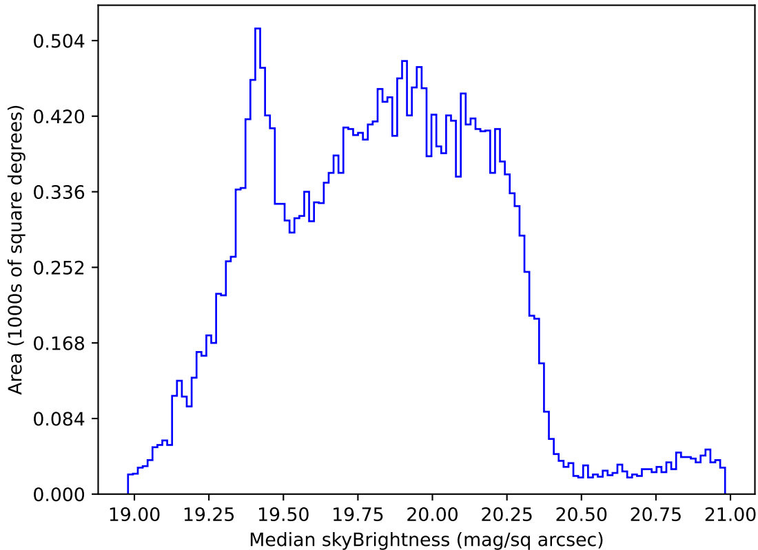
too_elab_heavy_r64_d2_griz_v3.4_10yrs Yr 1 all bands: Median skyBrightness
