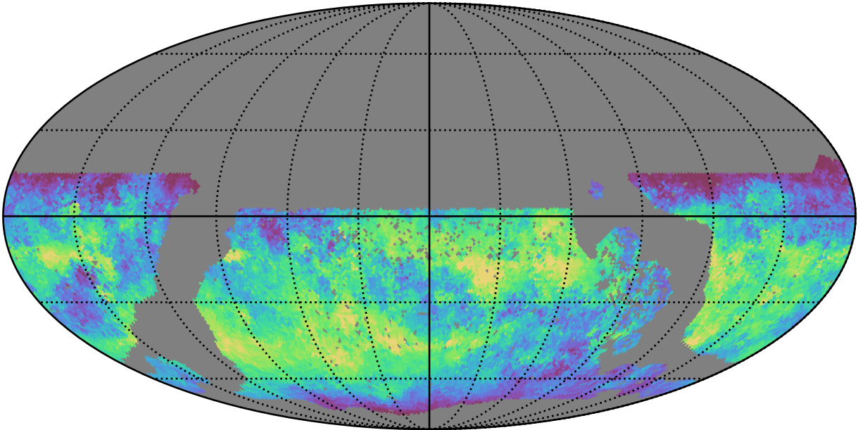
too_elab_heavy_r64_d2_griz_v3.4_10yrs WFD z band: Median skyBrightness
