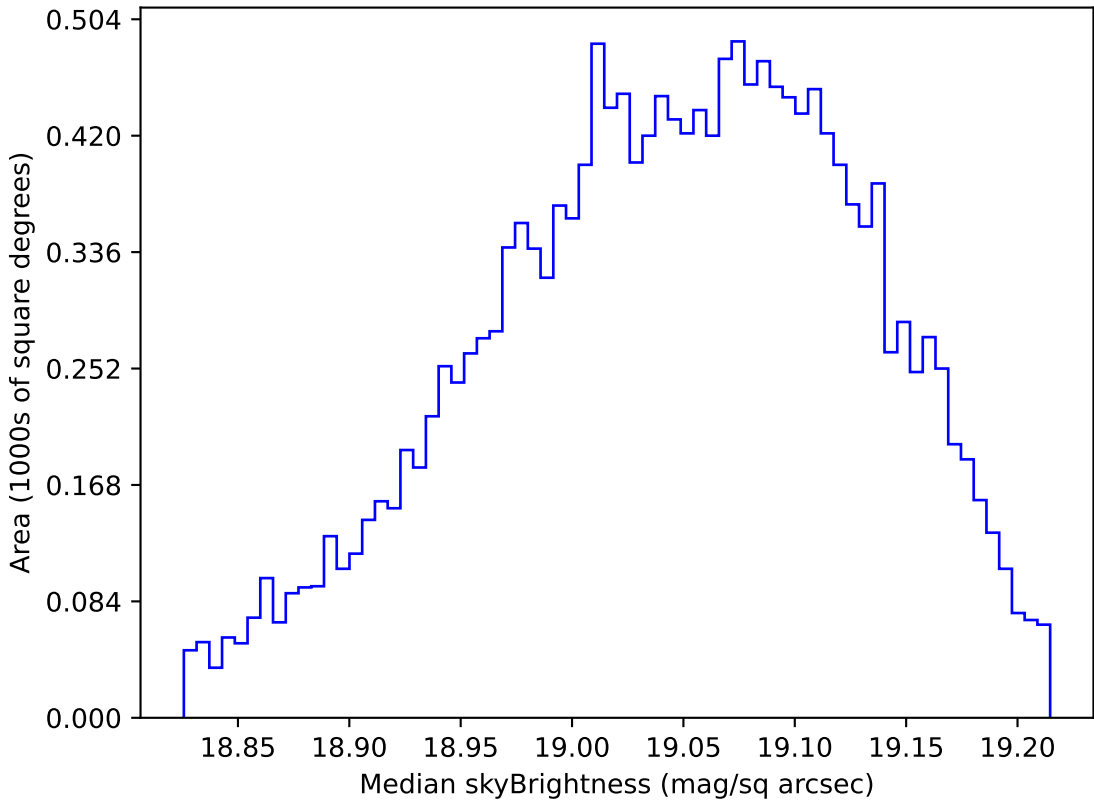
too_elab_heavy_r64_d2_griz_v3.4_10yrs WFD z band: Median skyBrightness
