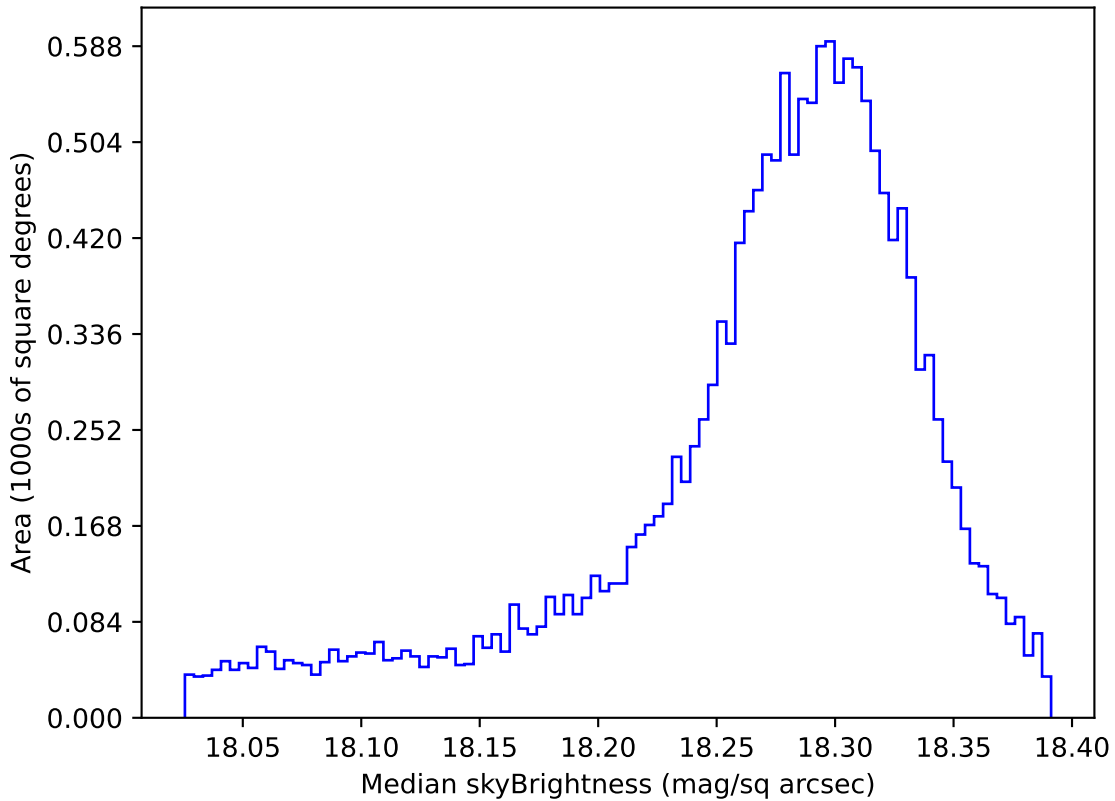
too_elab_heavy_r64_d2_griz_v3.4_10yrs WFD y band: Median skyBrightness
