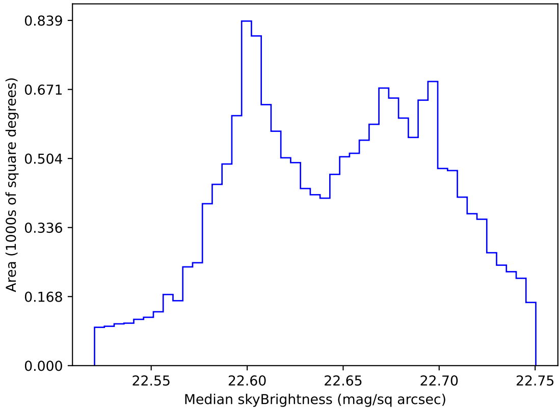
too_elab_heavy_r64_d2_griz_v3.4_10yrs WFD u band: Median skyBrightness
