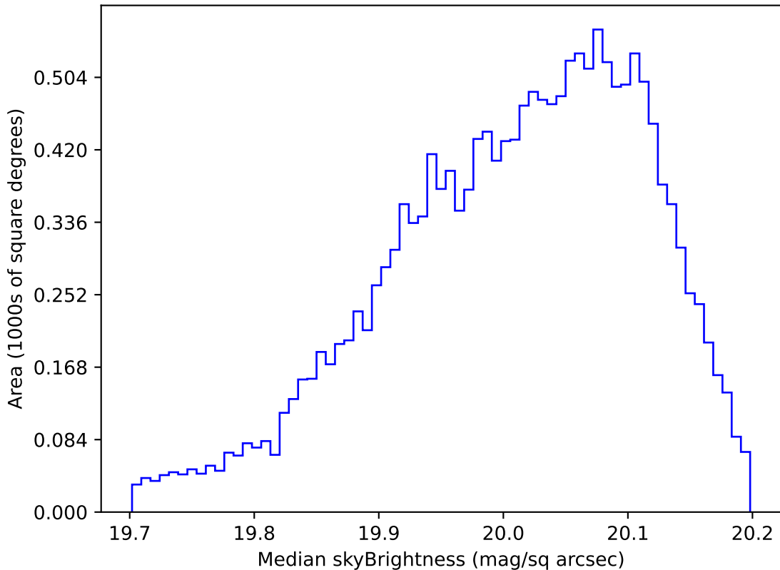
too_elab_heavy_r64_d2_griz_v3.4_10yrs WFD i band: Median skyBrightness
