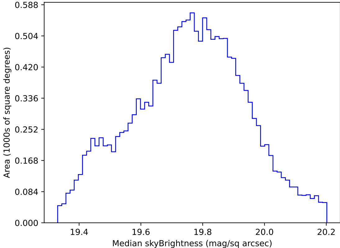
too_elab_heavy_r64_d2_griz_v3.4_10yrs WFD all bands: Median skyBrightness
