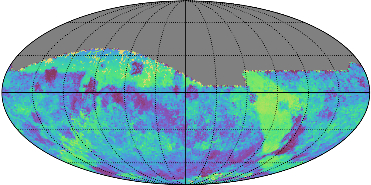
too_elab_heavy_r64_d2_griz_v3.4_10yrs All sky all bands: Median skyBrightness
