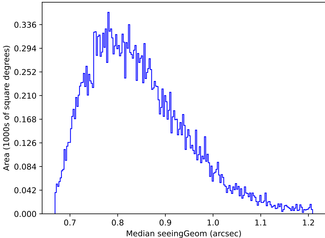
too_elab_heavy_r64_d2_griz_v3.4_10yrs Yr 1 z band: Median seeingGeom
