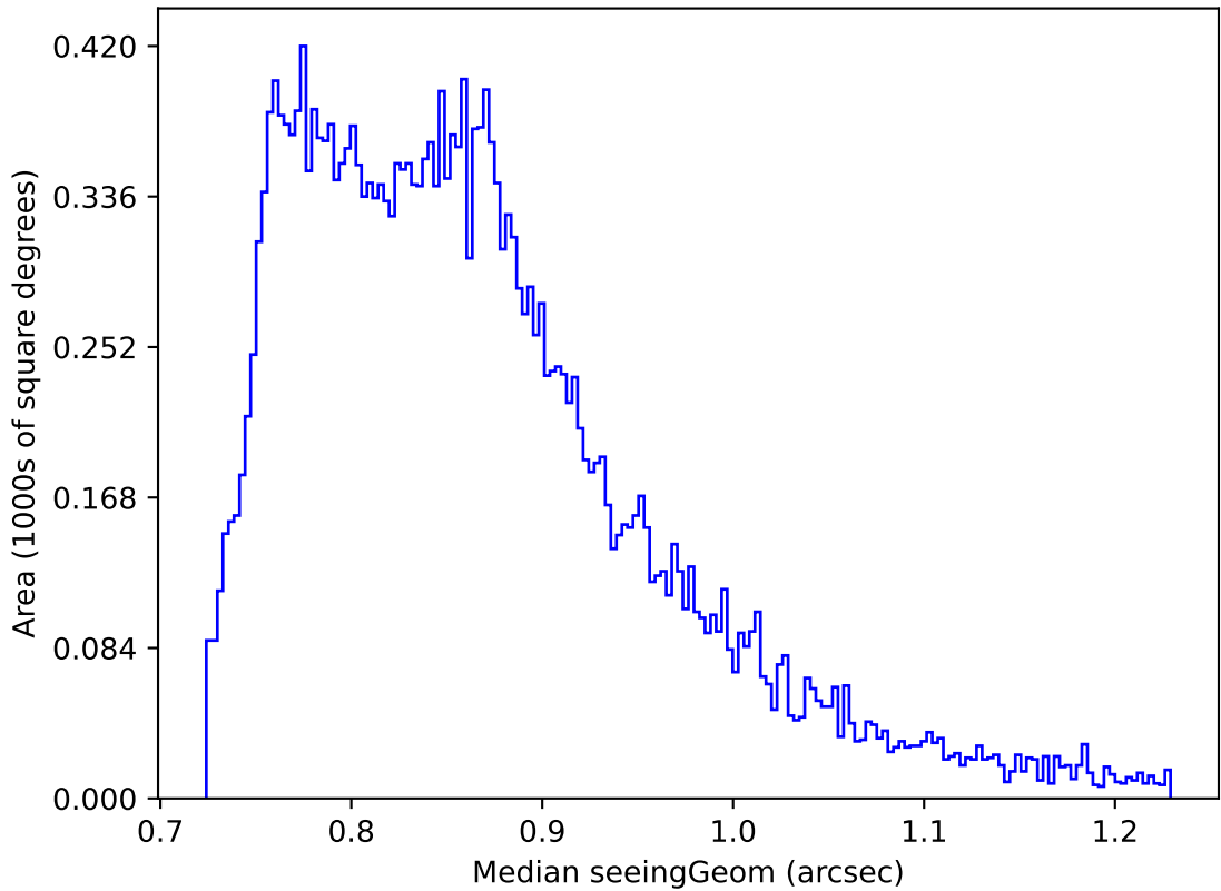
too_elab_heavy_r64_d2_griz_v3.4_10yrs Yr 1 all bands: Median seeingGeom
