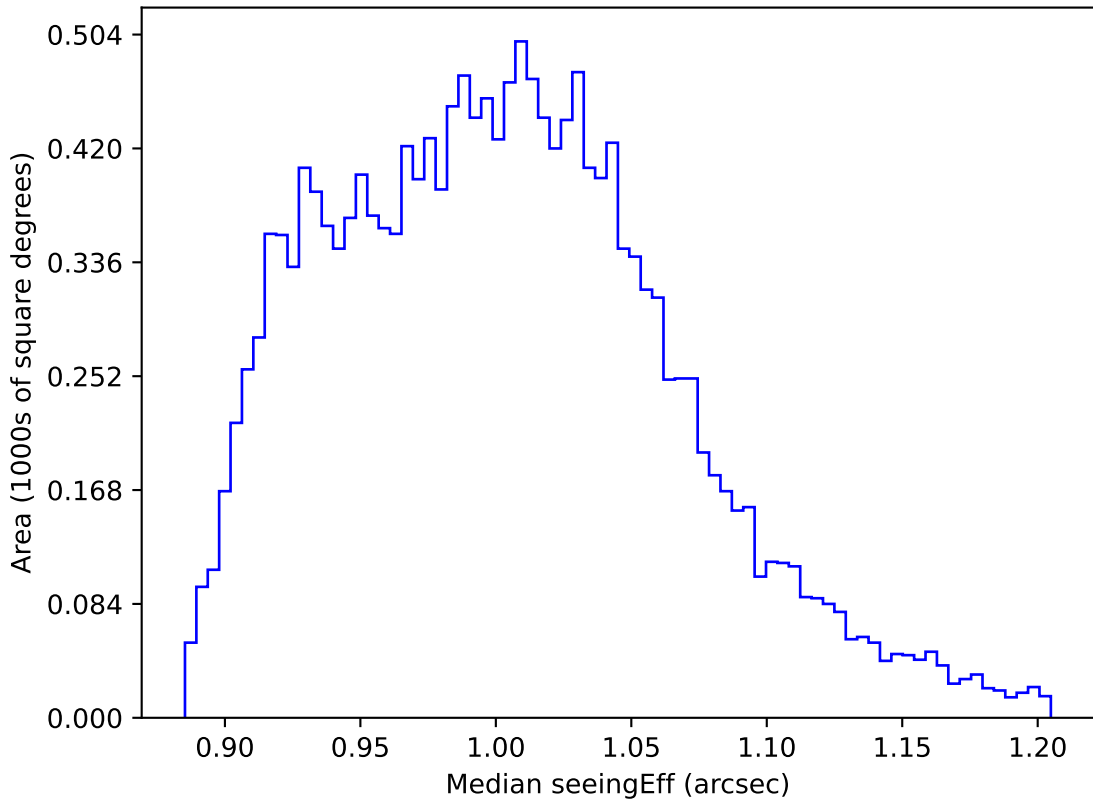
too_elab_heavy_r64_d2_griz_v3.4_10yrs WFD y band: Median seeingEff
