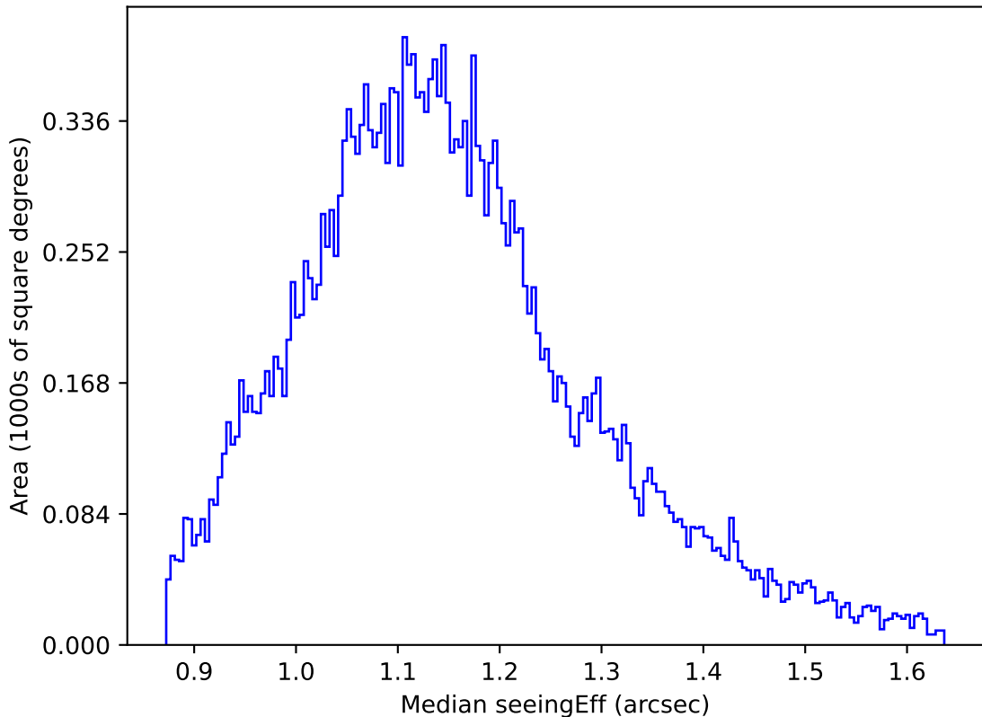
too_elab_heavy_r64_d2_griz_v3.4_10yrs All sky g band: Median seeingEff
