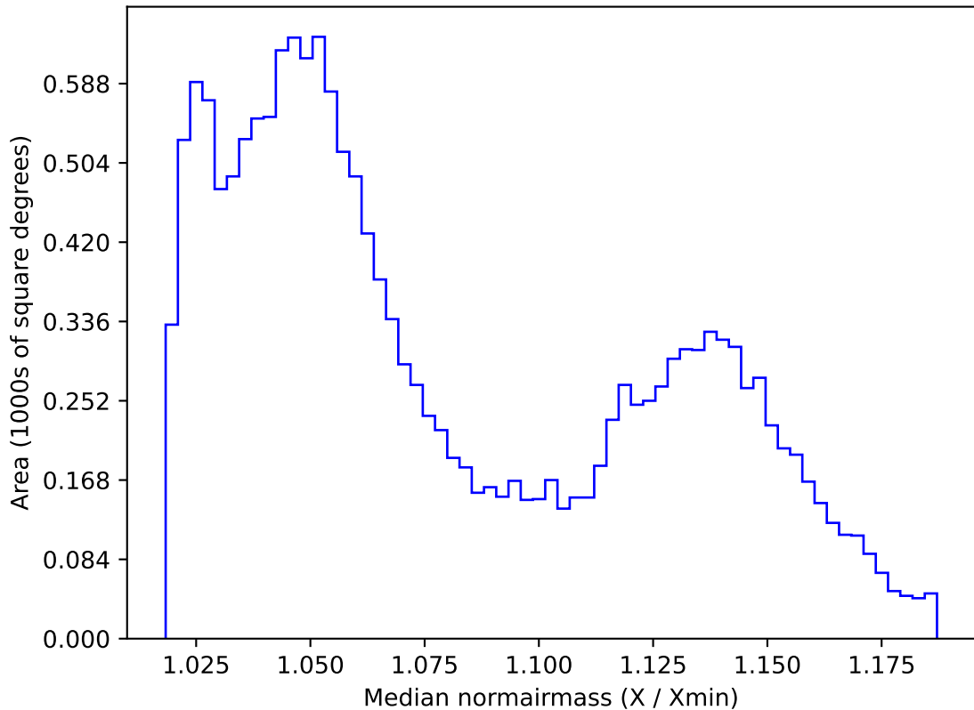
too_elab_heavy_r64_d2_griz_v3.4_10yrs WFD r band: Median normairmass
