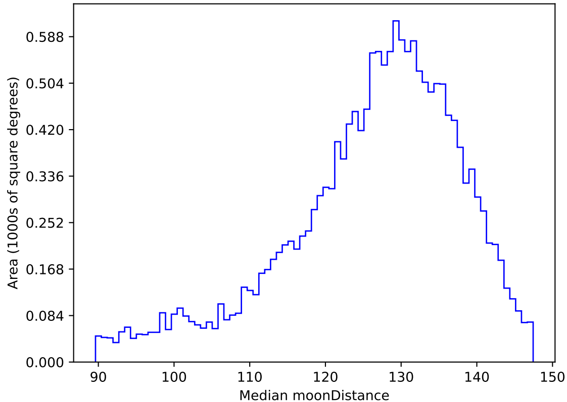
too_elab_heavy_r64_d2_griz_v3.4_10yrs WFD u band: Median moonDistance
