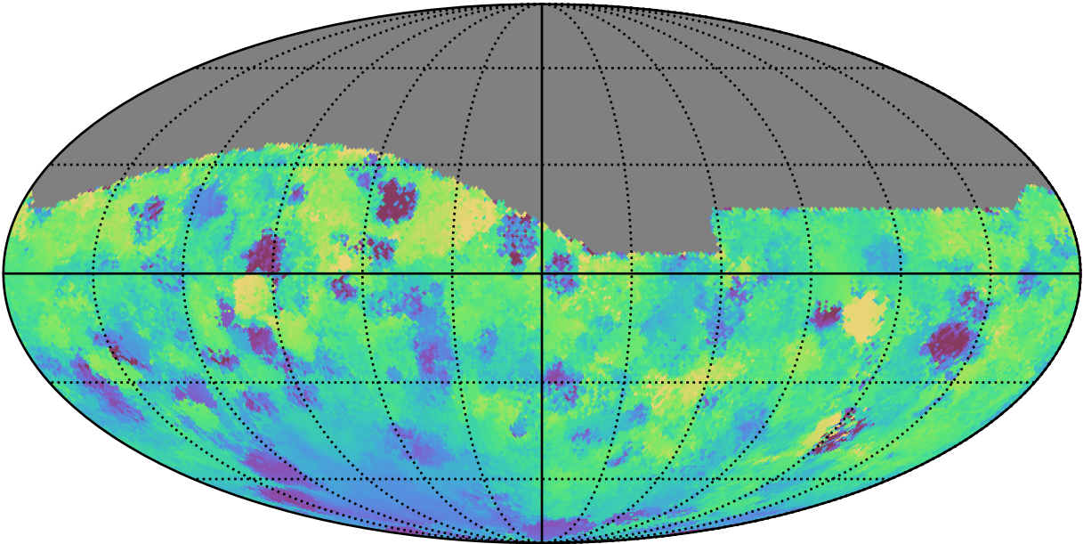
too_elab_heavy_r64_d2_griz_v3.4_10yrs All sky g band: Median moonDistance
