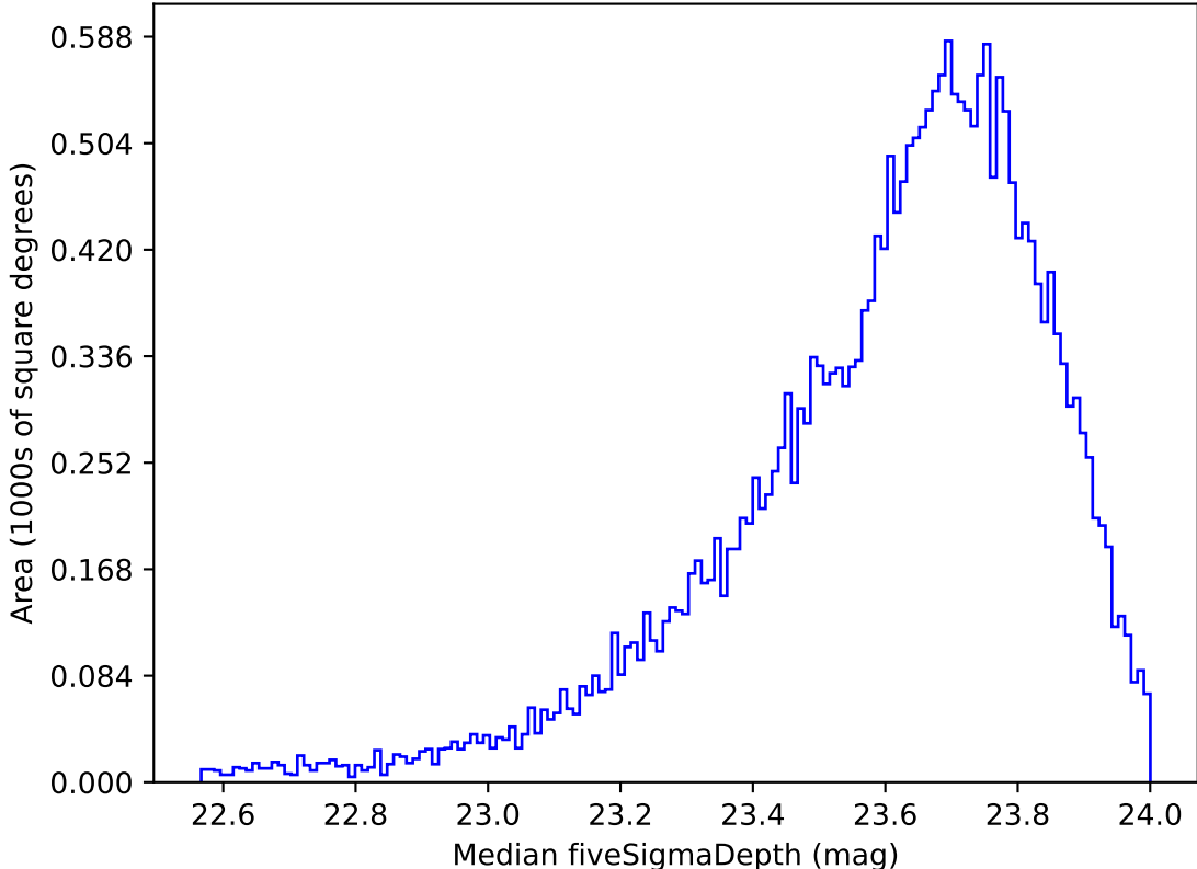
too_elab_heavy_r64_d2_griz_v3.4_10yrs Yr 1 i band: Median fiveSigmaDepth
