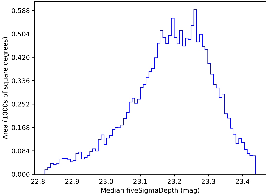
too_elab_heavy_r64_d2_griz_v3.4_10yrs WFD u band: Median fiveSigmaDepth
