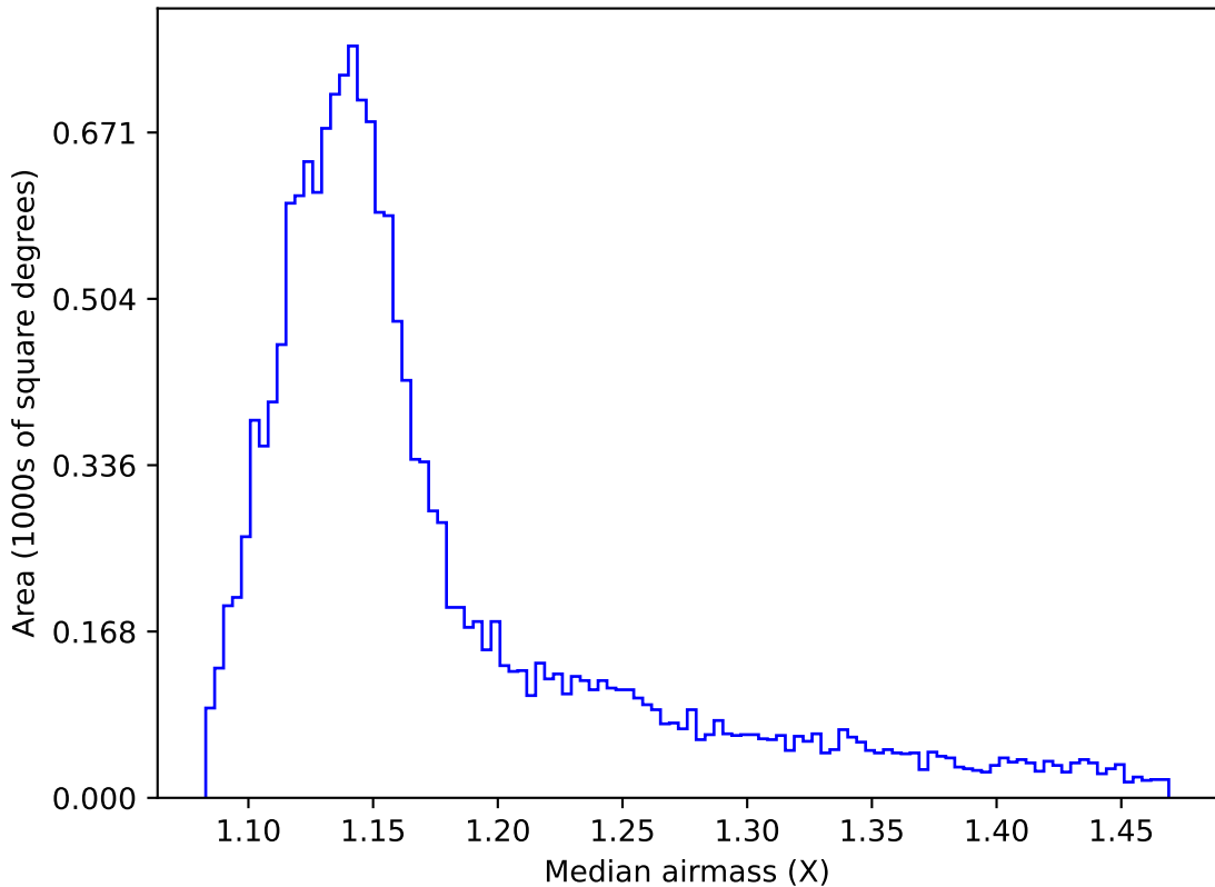
too_elab_heavy_r64_d2_griz_v3.4_10yrs WFD i band: Median airmass
