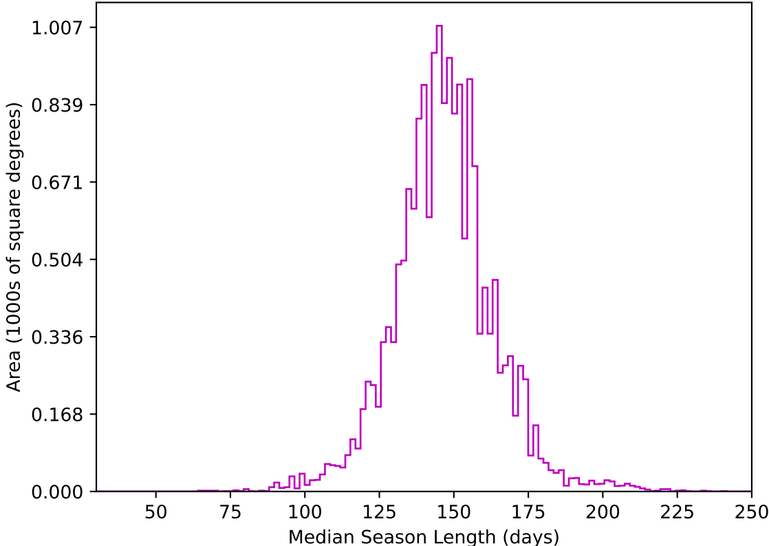
too_elab_heavy_r64_d2_griz_v3.4_10yrs WFD z band: Median Season Length
