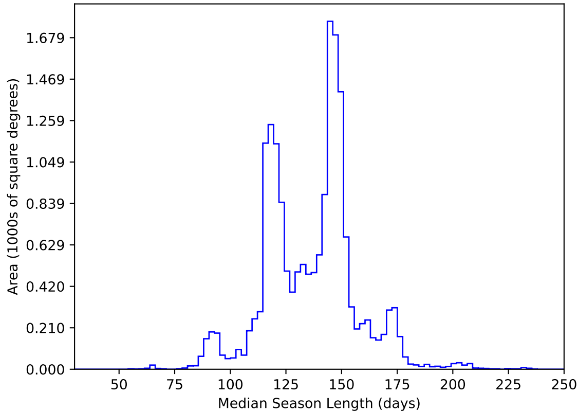
too_elab_heavy_r64_d2_griz_v3.4_10yrs WFD y band: Median Season Length
