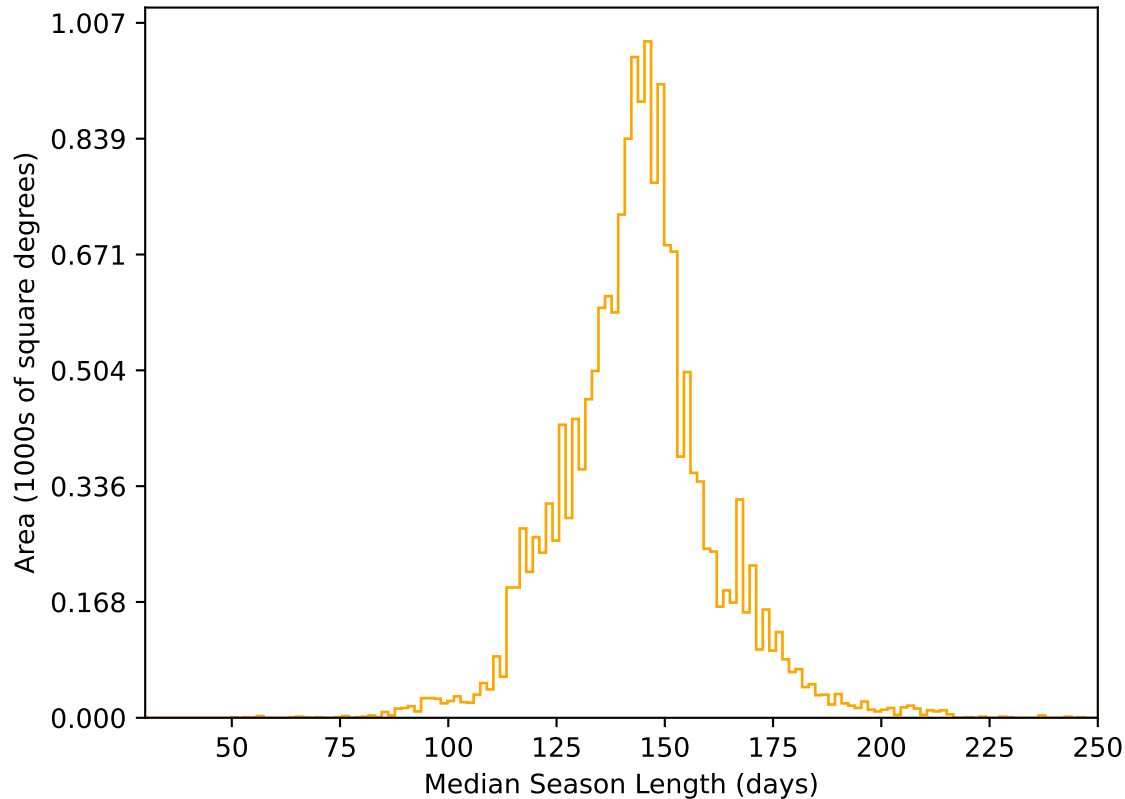
too_elab_heavy_r64_d2_griz_v3.4_10yrs WFD r band: Median Season Length
