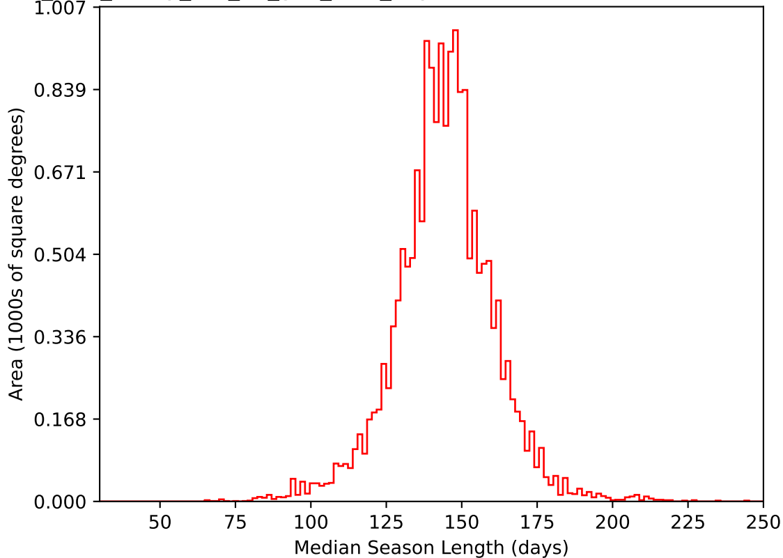
too_elab_heavy_r64_d2_griz_v3.4_10yrs WFD i band: Median Season Length
