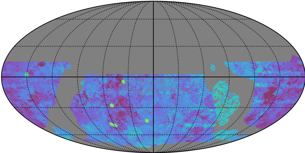
too_elab_heavy_r64_d2_griz_v3.4_10yrs WFD g band: Median Season Length
