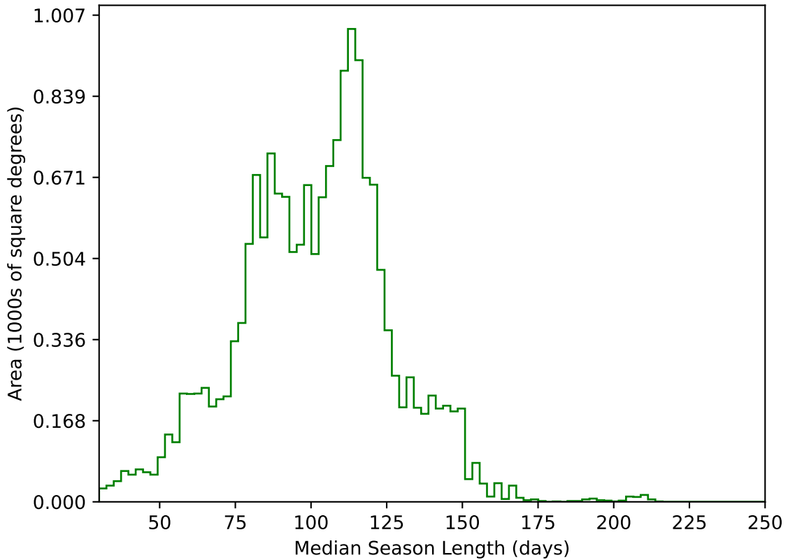
too_elab_heavy_r64_d2_griz_v3.4_10yrs WFD g band: Median Season Length
