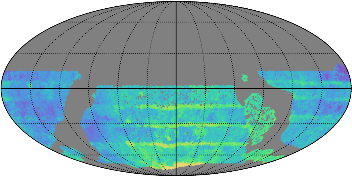
too_elab_heavy_r64_d2_griz_v3.4_10yrs WFD all bands: Median Season Length
