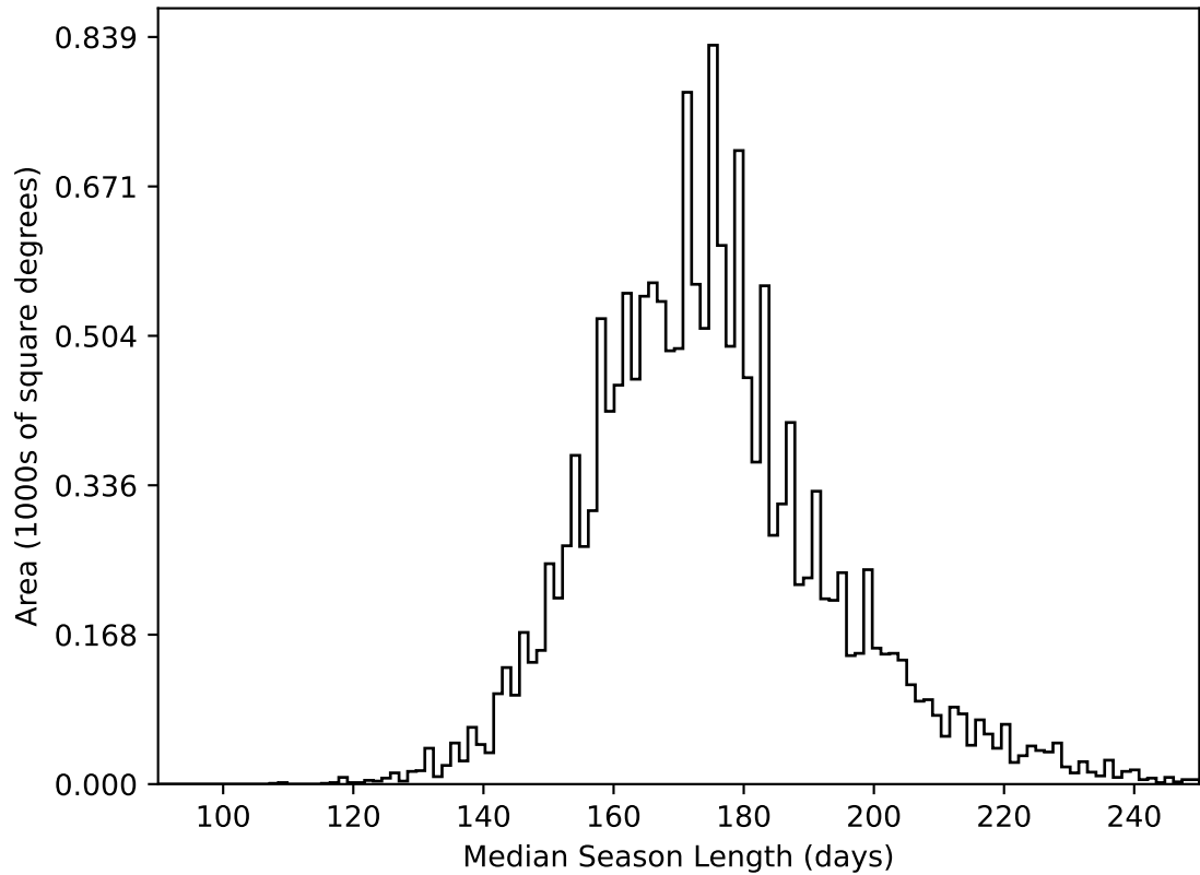
too_elab_heavy_r64_d2_griz_v3.4_10yrs WFD all bands: Median Season Length
