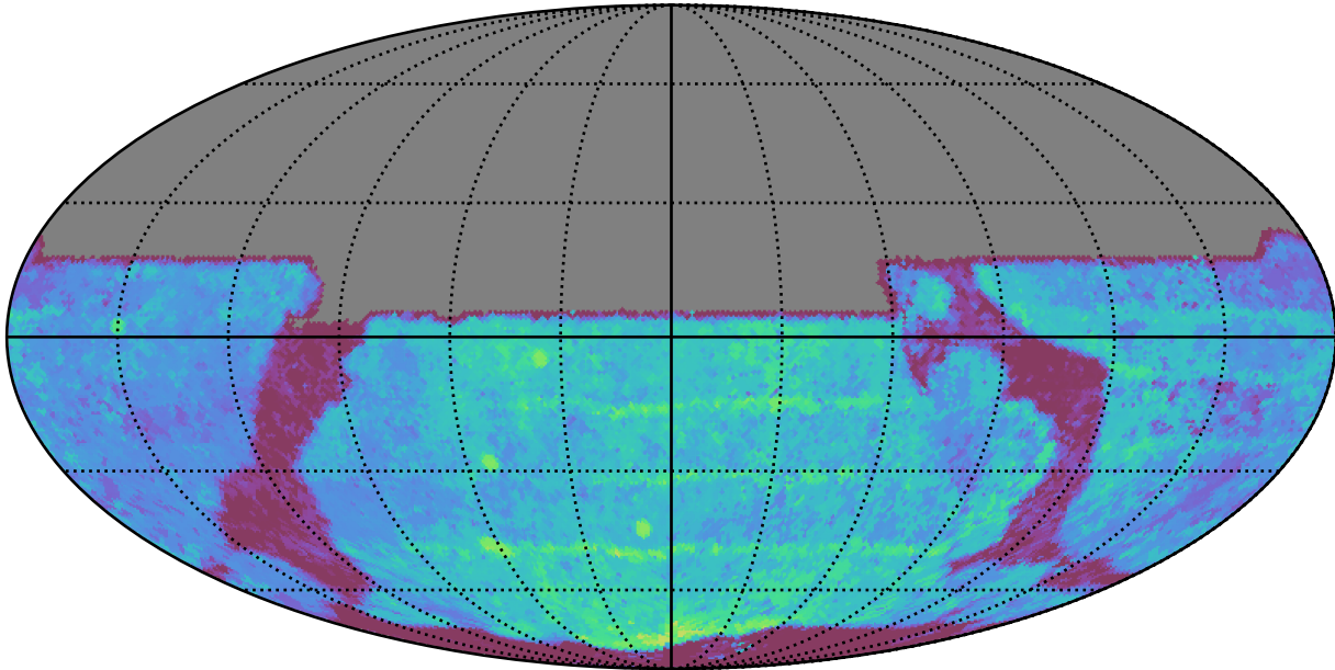
too_elab_heavy_r64_d2_griz_v3.4_10yrs All sky y band: Median Season Length
