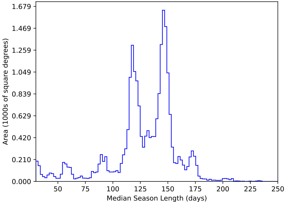
too_elab_heavy_r64_d2_griz_v3.4_10yrs All sky y band: Median Season Length
