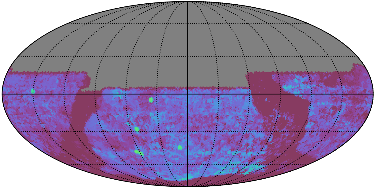
too_elab_heavy_r64_d2_griz_v3.4_10yrs All sky u band: Median Season Length
