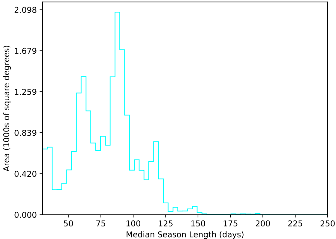
too_elab_heavy_r64_d2_griz_v3.4_10yrs All sky u band: Median Season Length
