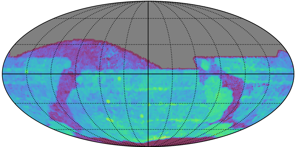
too_elab_heavy_r64_d2_griz_v3.4_10yrs All sky r band: Median Season Length
