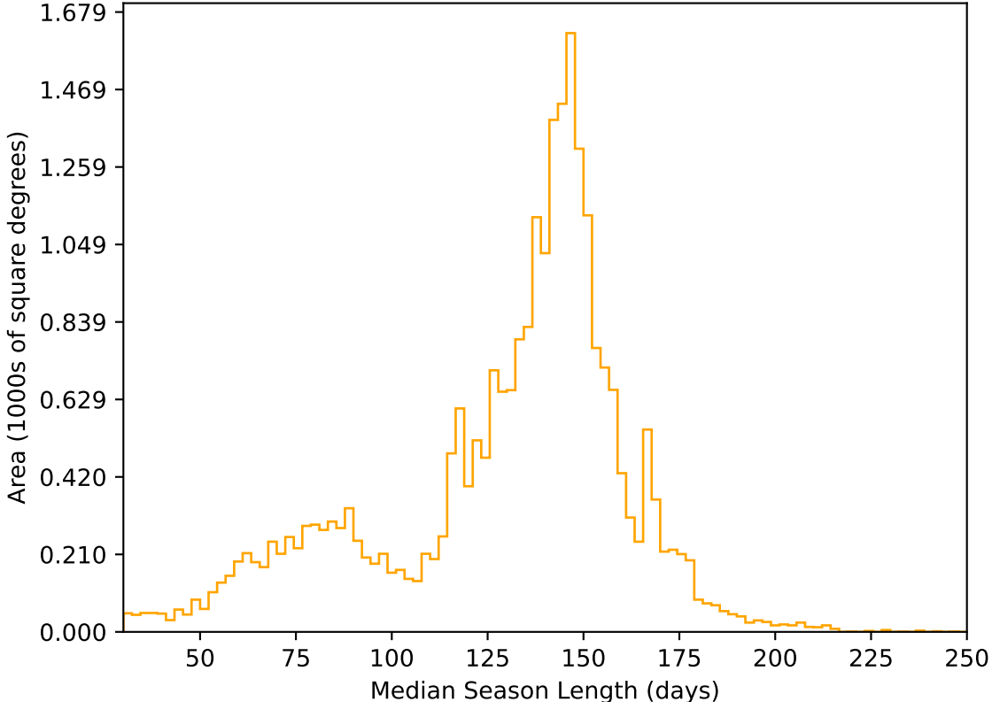
too_elab_heavy_r64_d2_griz_v3.4_10yrs All sky r band: Median Season Length
