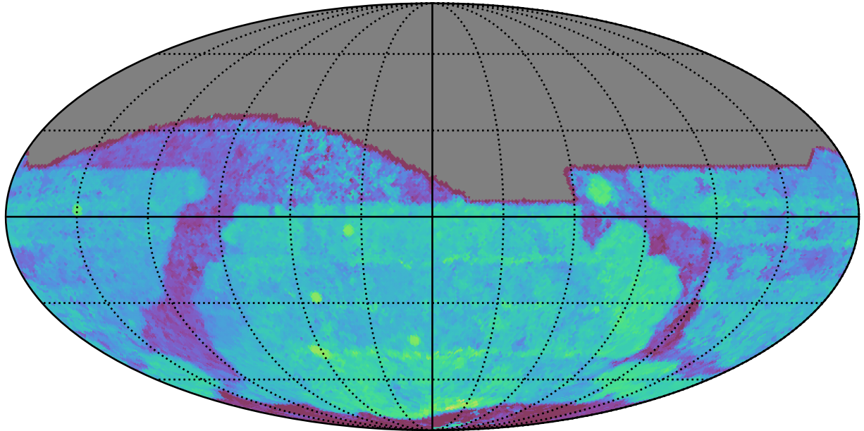
too_elab_heavy_r64_d2_griz_v3.4_10yrs All sky i band: Median Season Length
