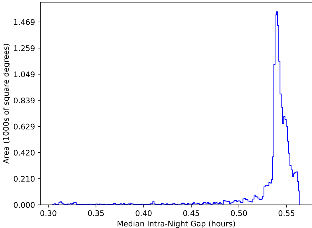
too_elab_heavy_r64_d2_griz_v3.4_10yrs WFD: Median Intra-Night Gap
