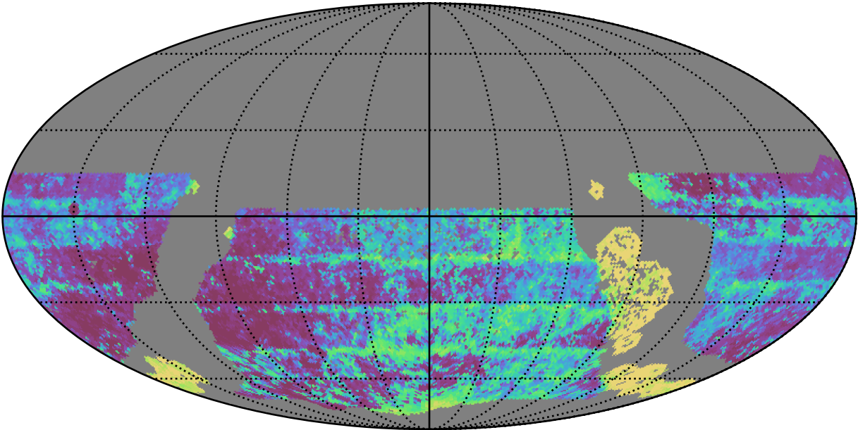
too_elab_heavy_r64_d2_griz_v3.4_10yrs WFD y band: Median Inter-Night Gap
