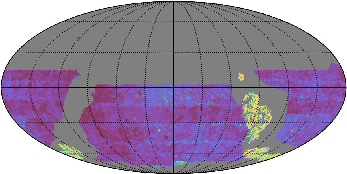
too_elab_heavy_r64_d2_griz_v3.4_10yrs WFD u band: Median Inter-Night Gap
