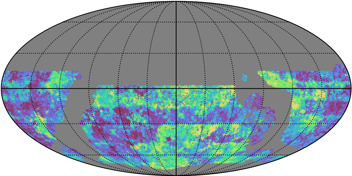
too_elab_heavy_r64_d2_griz_v3.4_10yrs WFD g band: Median Inter-Night Gap
