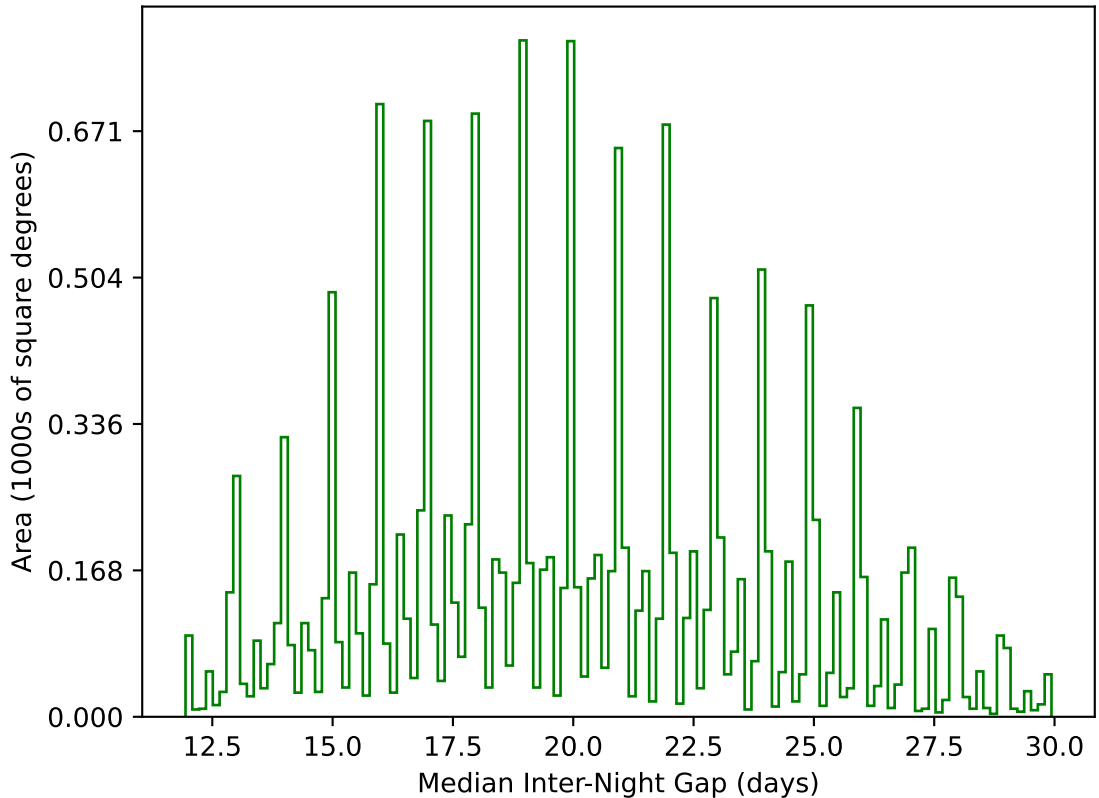
too_elab_heavy_r64_d2_griz_v3.4_10yrs WFD g band: Median Inter-Night Gap
