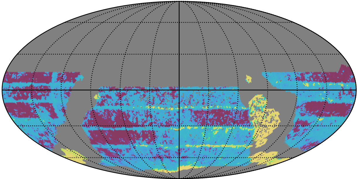
too_elab_heavy_r64_d2_griz_v3.4_10yrs WFD all bands: Median Inter-Night Gap
