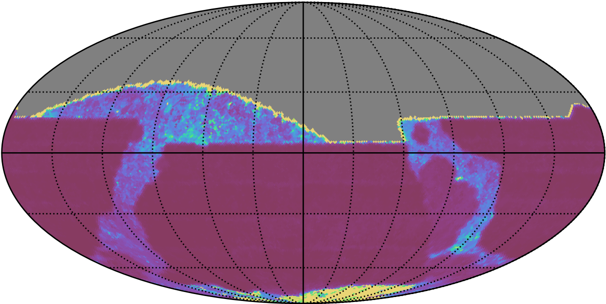
too_elab_heavy_r64_d2_griz_v3.4_10yrs All sky z band: Median Inter-Night Gap
